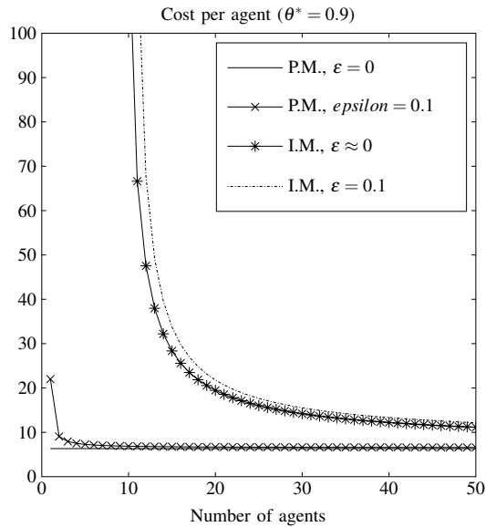
Fig. 3. Cost per agent in the basic example with noisy dynamics and observations (P.M.=perfect measurements, I.M.=imperfect measurements, A=0 ). In the case \epsilon = 0.1 and noisy observations, the cost is infinite for less than 10 agents.
