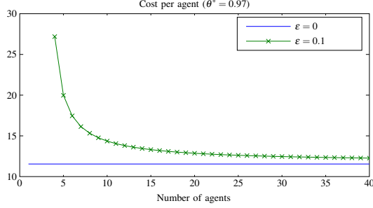
Fig. 2. Cost per agent in the basic example with noisy dynamics, under perfect measurements. The cost is infinite for less than 4 agents.
