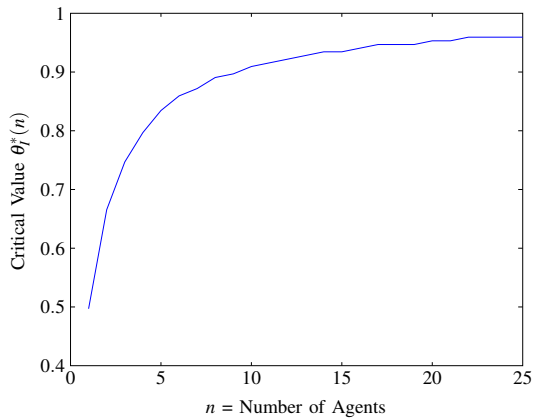
Fig. 4. Evolution of \theta_c^*(n) with the number of agents in the basic example ( \epsilon \approx 0 , A=0 ).
